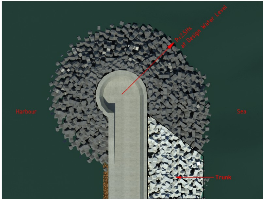
Plan View Typical Breakwater Head
