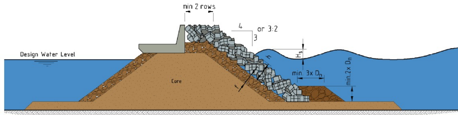
Cross Section Typical Breakwater Head
